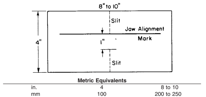
FIG. 2 Illustration of Modified Grab Test Specimens
