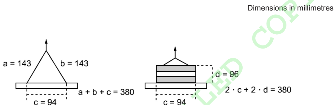
Figure A.2 — Example of the same cord on the same toy measured with the 2 different test procedures
