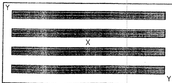
Figure B.2 — Measurement of irradiance uniformity in devices with a flat specimen plane (shaded areas indicate light sources)
