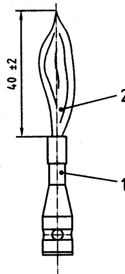
d) Vertical stand-by flame height
