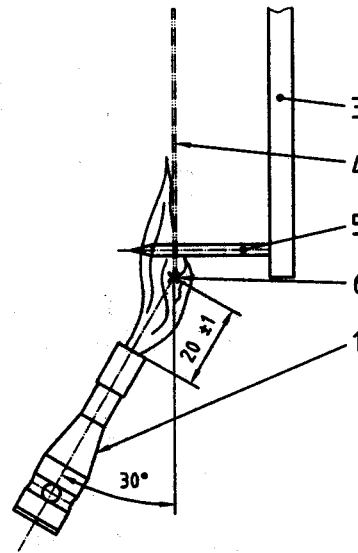
b) Bottom-edge ignition
