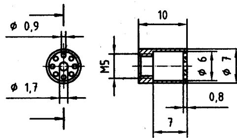
c) Flame stabilizer
